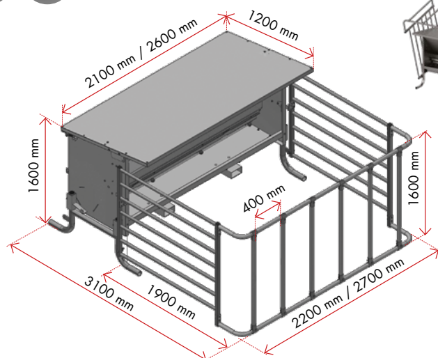
Cabina inclinabile
